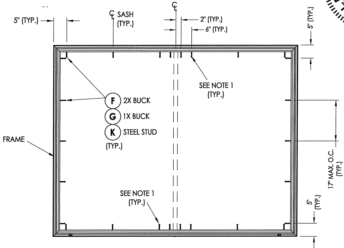
FRAME ANCHORING
