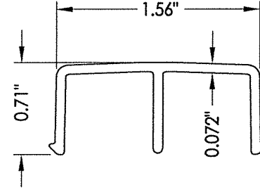
4 SILL TRACK
