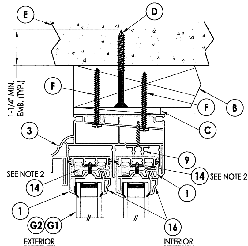
4 VERTICAL CROSS SECTION 2 2X Buck Masonry Construction
